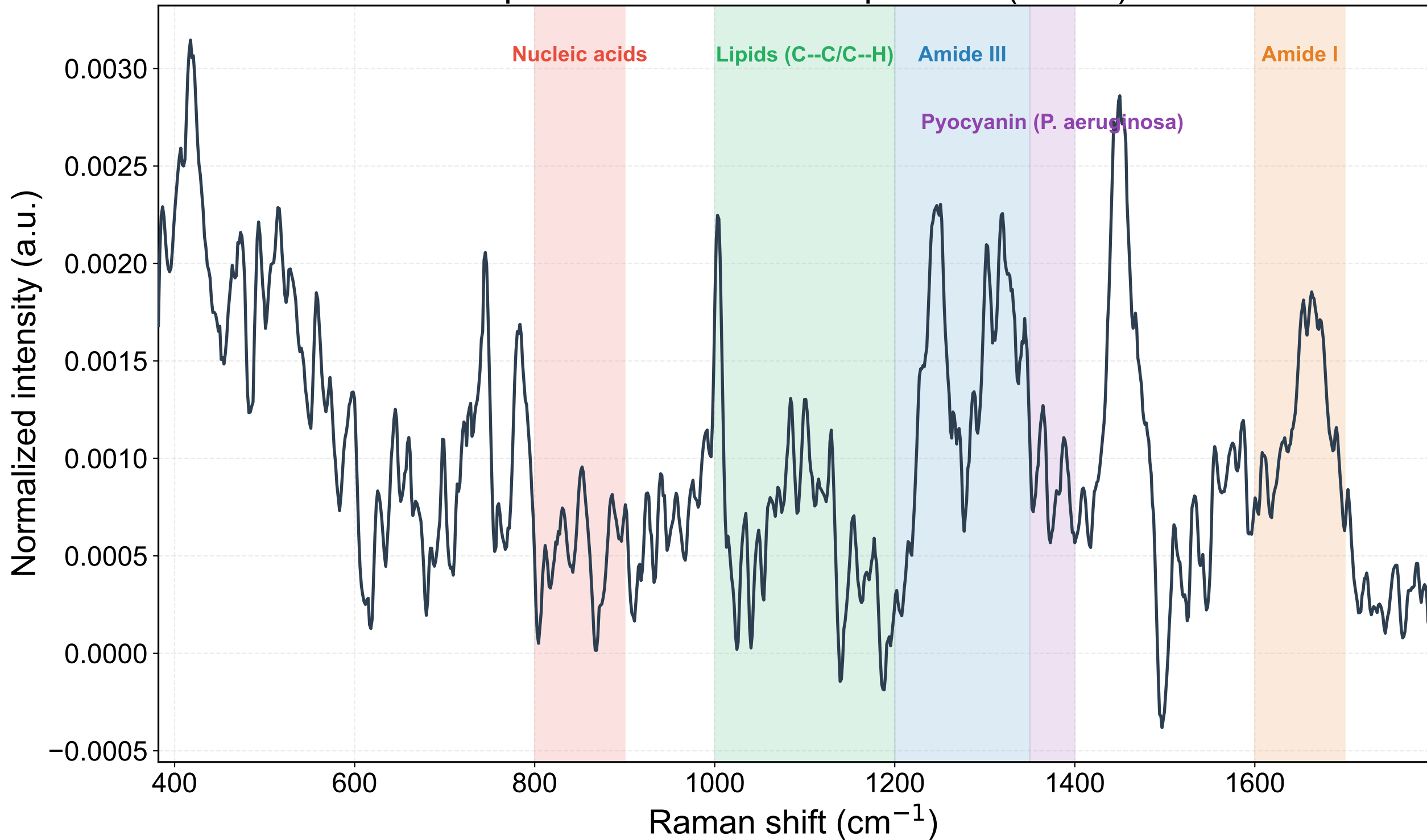
Representative Raman Spectrum (E. coli)
